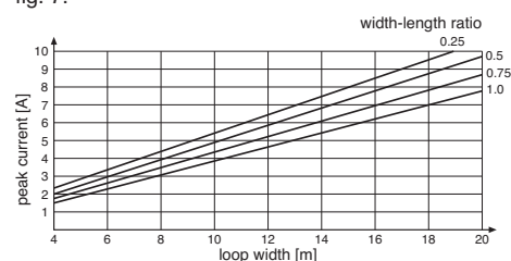
Fig. 7 Peak current in the induction loop
