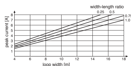
Fig. 7 Peak current in the induction loop
