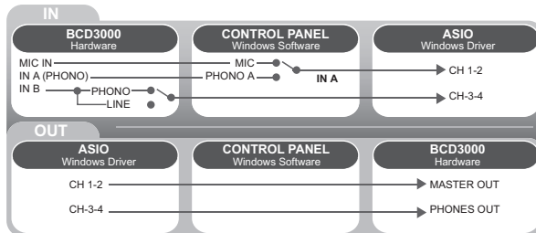
Abb. 5.3: Audio routing in STANDARD mode (ASIO driver)
