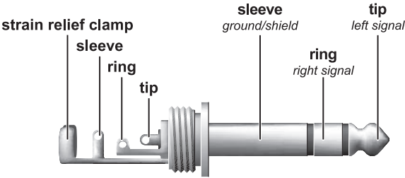
Fig. 7.2: 1/4" TRS headphones connector
