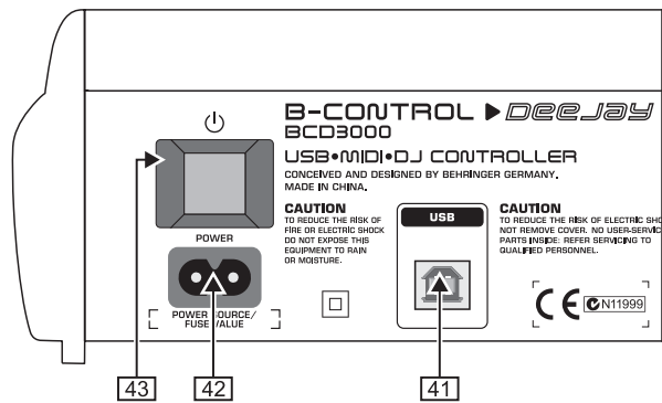
Fig. 3.3: POWER switch, mains and USB connectors
