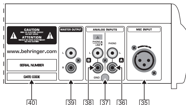
Fig. 3.2: The rear-panel audio connectors of the BCD3000
