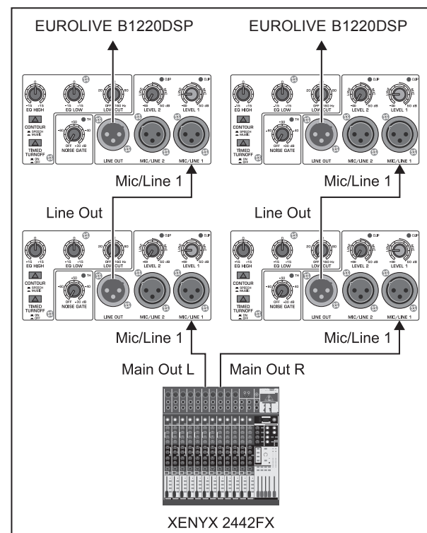
Fig. 4.3: Linking several B1220DSP speakers
