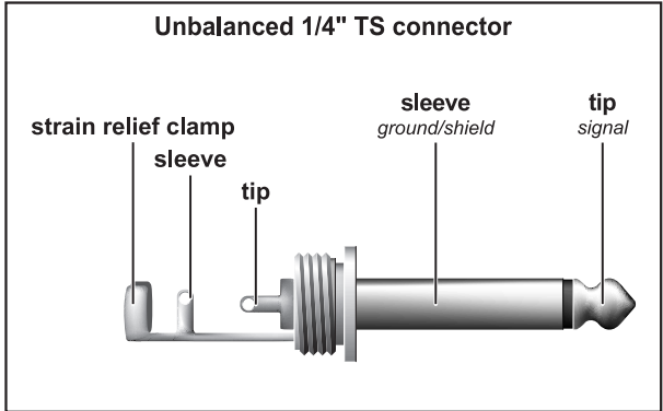
Fig. 4.3: 1/4" TS connector
