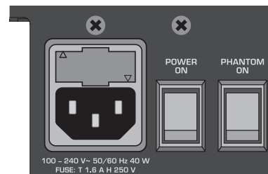
Fig. 2.16: Voltage supply and fuse
