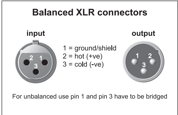
Fig. 4.2: XLR connections
