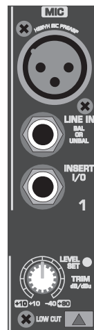
Fig. 2.1: Connectors and controls of mic/line inputs
