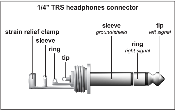
Fig. 4.6: 1/4" TRS connector for headphones
