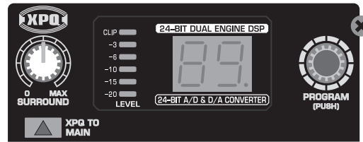
Fig. 3.3: Digital Effects module and XPQ Surround Function control elements
