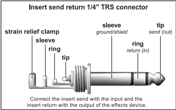
Fig. 4.5: Insert send return 1/4" TRS connector
