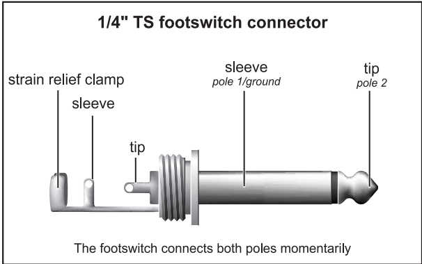
Fig. 4.1: 1/4" TS footswitch connector
