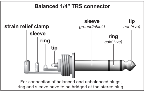
Fig. 4.4: 1/4" TRS connector
